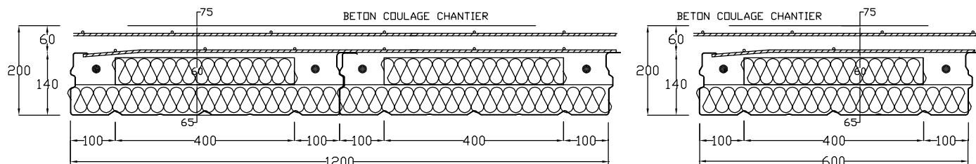
COFRADAL 230 PAC
