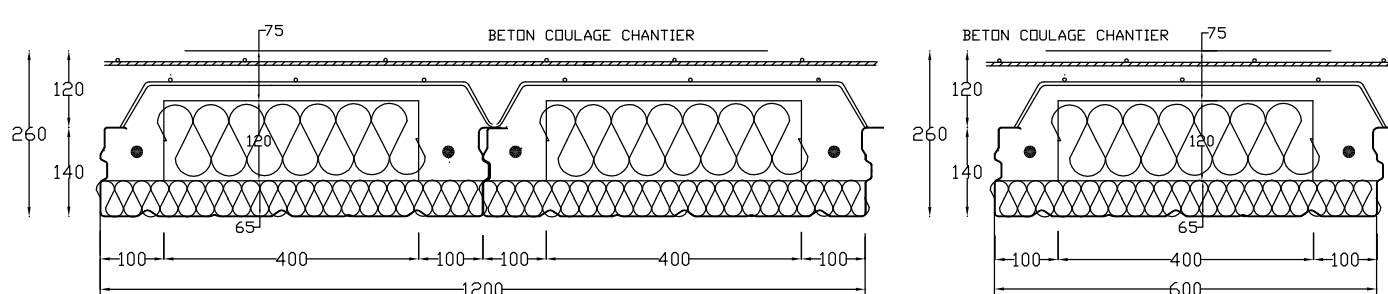
COFRADAL 260 PAC
