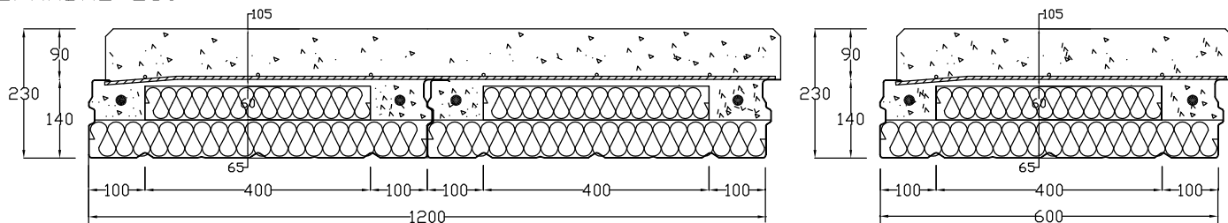
COFRADAL 230
