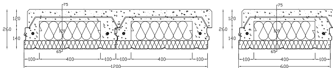
COFRADAL 260
