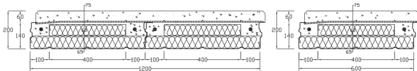
COFRADAL 200
