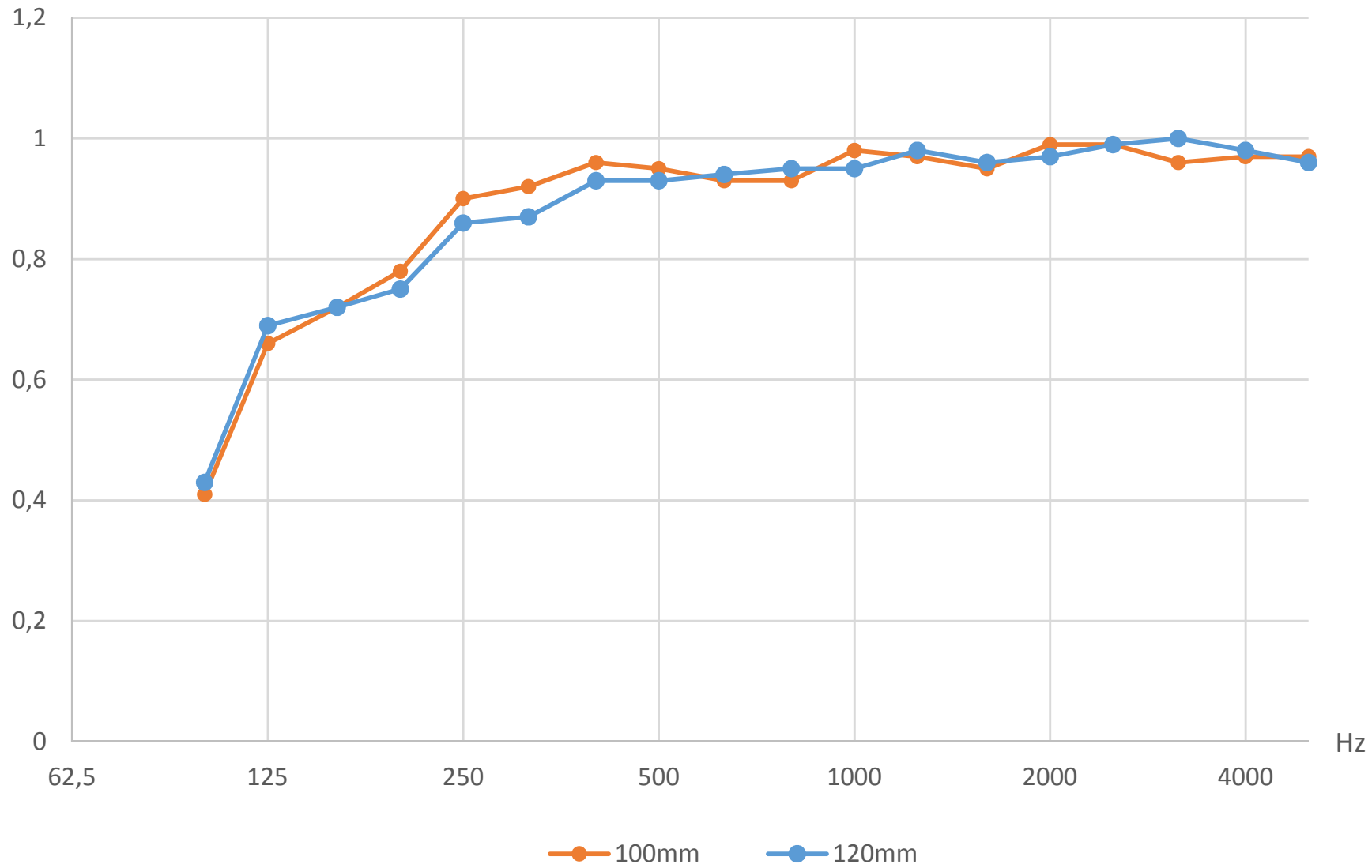
Acoustic absorption, comparison 100mm / 120mm wall glasswool, 0,6/0,6 1-side perforated
