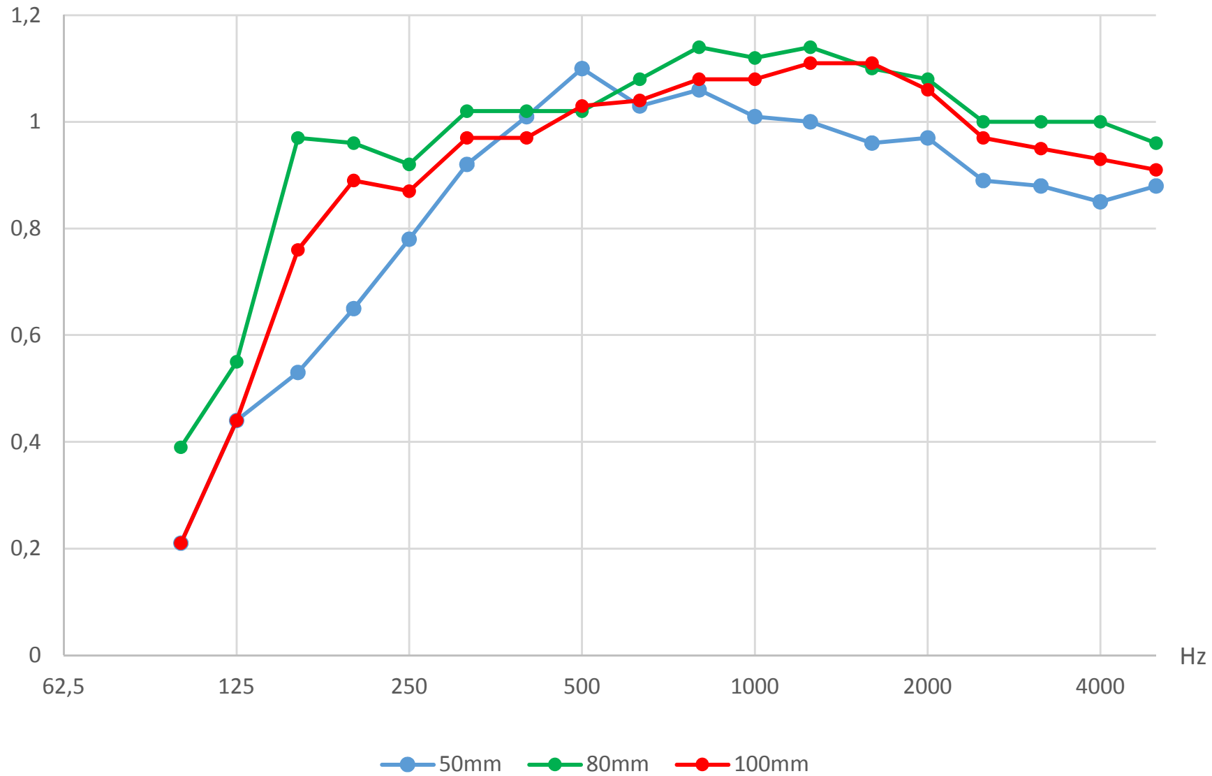
Acoustic absorption, comparison 50 / 80 / 100 mm roof, rockwool 0,6/0,6 inside perforated
