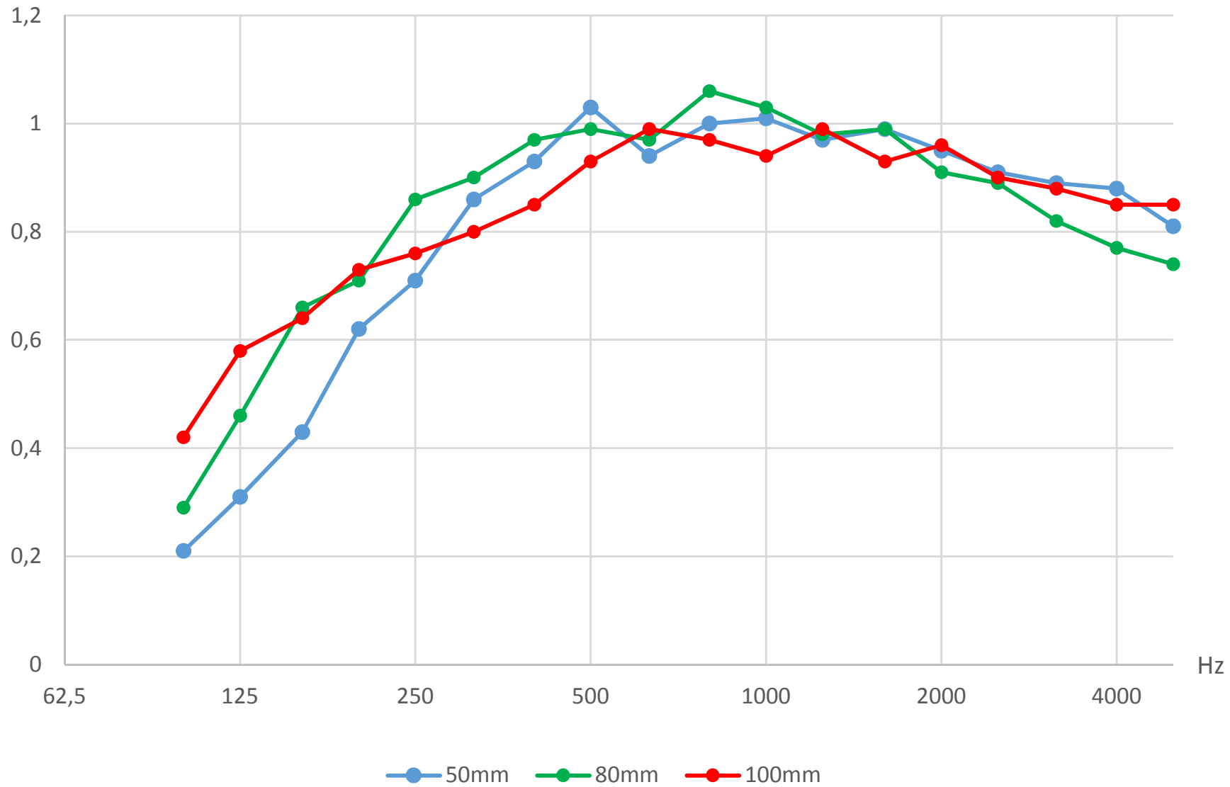
Acoustic absorption, comparison 50 / 80 / 100 mm wall, rockwool, 0,6/0,6 1-side perforated
