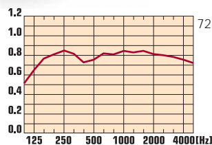
delta sans Isolation h 439 mm
