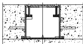
2. Pouring of the concrete
