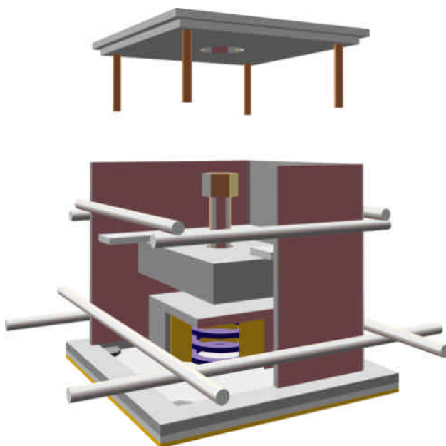
Exploded 3D view of ISO-MONT-LF-150 box
