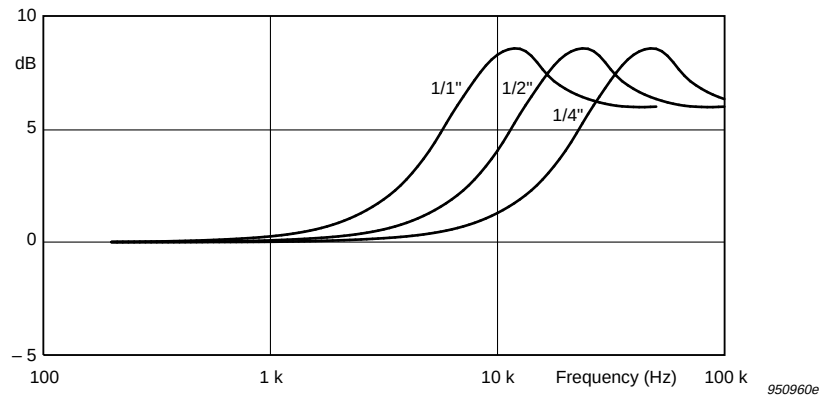
Fig.2.28 Ratio between the pressure at the diaphragm position and the pressure of the undisturbed sound field. The same pressure changes occur for bodies of larger and smaller body diameter, but the frequency range is shifted and is inversely proportional to the diameter of the microphone body
