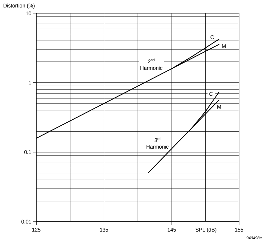
Fig.2.24 Distortion of microphone (M) and of microphone-preamplifier combination (C). The preamplifier distortion which plays the minor role is just noticeable at the highest measurable levels. The distortion is valid for a free-field microphone ( \frac{1}{2} ", 50 mV/Pa). It is measured at 90 Hz and is representative for that part of the frequency range where the diaphragm displacement is dominantly controlled by stiffness
