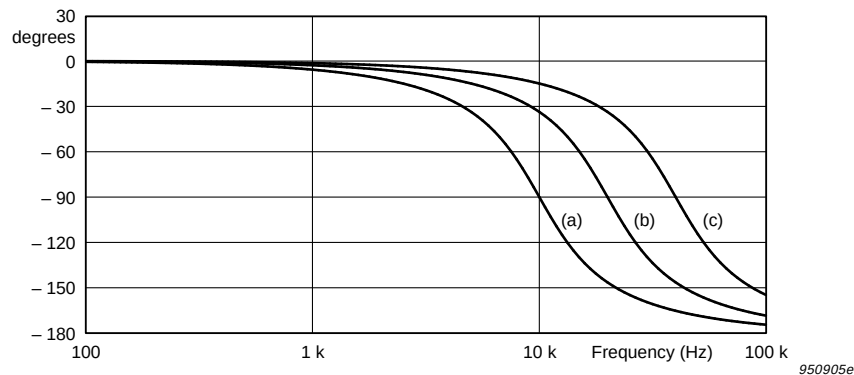
Fig.2.12 Phase of frequency responses (pressure). The curves are valid for models of microphone with critical damping and different diaphragm diameters (relative scale: 1 (a), 0.5 (b), 0.25 (c)). The numbers chosen for the calculation approximate the parameters of existing 1", \frac{1}{2} " and \frac{1}{4} " microphones
