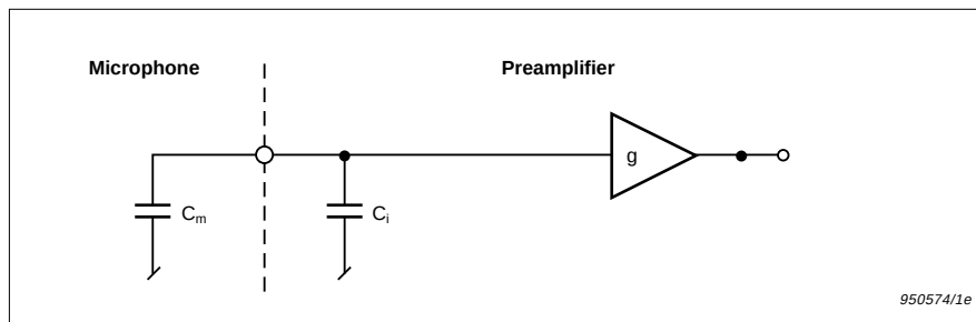
Fig.3.2 Circuit diagram of preamplifier and microphone combination
