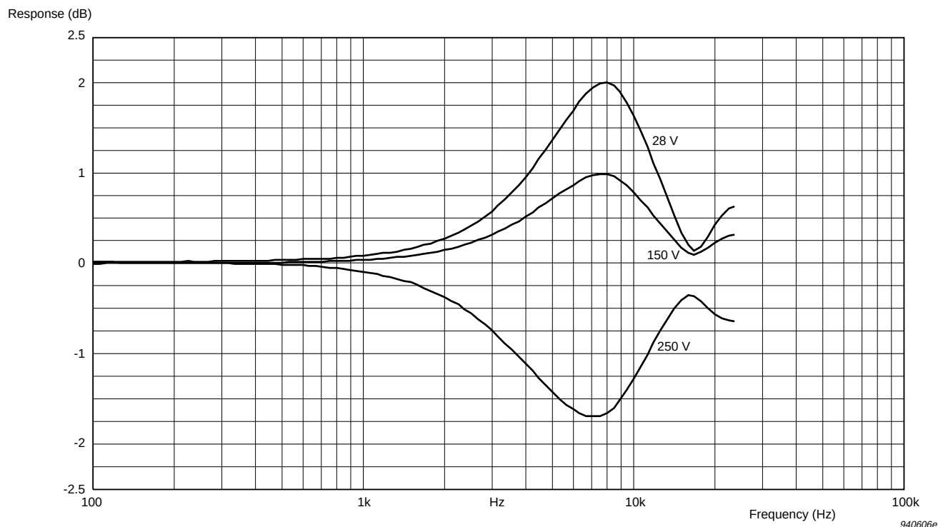
Fig.3.7 Example of the frequency response dependency with polarisation voltage. The curves are normalised to the nominal value of 200 V. This example is for a \frac{1}{2} " microphone with high sensitivity. The dependency is less for \frac{1}{2} " microphones with lower sensitivity
