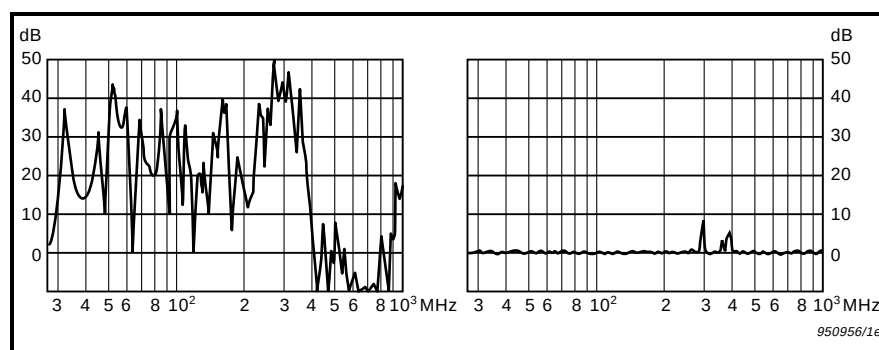
Fig.4.10 Preamplifier noise when exposed to electromagnetic field, before (left) and after EMC improvements (right). The 0 dB line corresponds to the inherent noise level of the preamplifier. The x-axis corresponds to the carrier frequency (20 MHz to 1 GHz)
