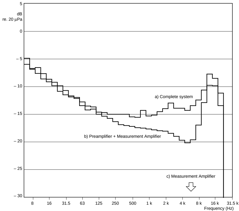
Fig.2.23 Equivalent levels of inherent noise (1/3 octave bandwidth) produced by the elements of a low noise system with a special 1" free-field microphone (100 mV/Pa and low diaphragm damping). The microphone and the preamplifier (20 dB gain) which contains a frequency response equalization network, form the main noise sources. The system noise level is -2 dB (A)
