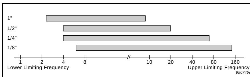
Fig.5.1 Upper limiting frequency response of 4 typical measurement microphones of different sizes \frac{1}{8} ", \frac{1}{4} ", \frac{1}{2} " and 1"
