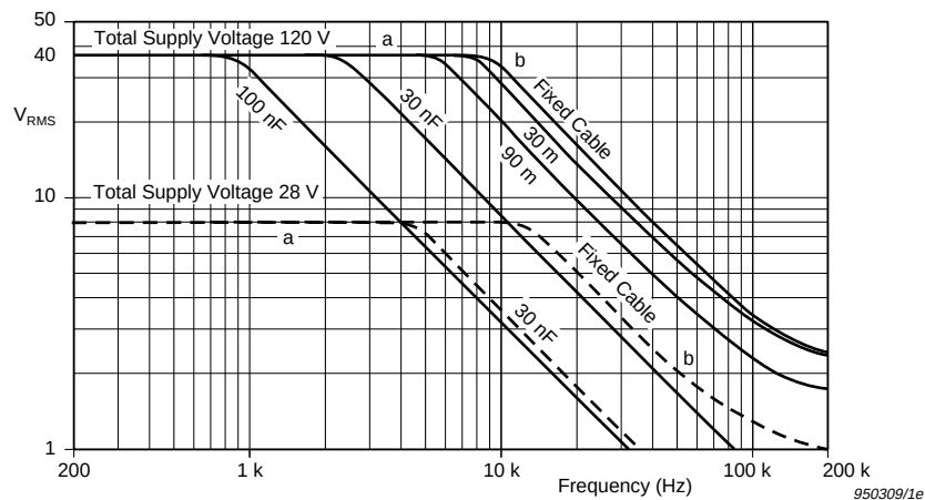
Fig.4.3 Maximum output voltage vs frequency showing the influence of preamplifier limitations caused by: a) maximum supply voltage, b) slew rate. The curves, for different cable lengths and loads, are all caused by current limitation
