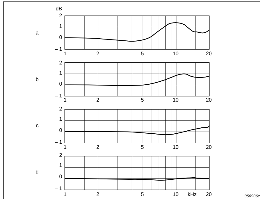
Fig.2.37 Differences between pressure and actuator responses for four different types of microphone: 1" pressure-field, 50 mV/Pa (a), 1" free-field, 50 mV/Pa (b), 1/2" pressure-field, 12.5 mV/Pa (c) and 1/2" free-field, 12.5 mV/Pa (d)
