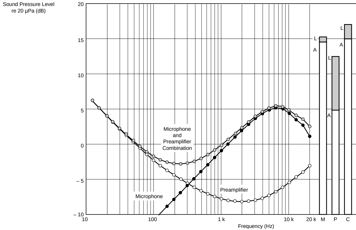
Fig.2.21 Third Octave Noise Spectra of a system consisting of a free-field microphone ( \frac{1}{2} " , 50 mV/Pa) and a high quality preamplifier. The electrical preamplifier noise dominates at low frequencies while Brownian movements of the microphone diaphragm create the most significant noise at high frequencies. The columns to the right show Linear (20 Hz – 20 kHz) (L) and A-weighted (A) noise levels for the microphone (M), preamplifier (P) and combination (C)
