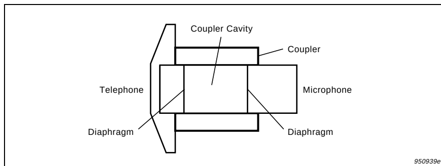
Fig.2.25 Schematic diagram of coupler used for headphone testing
