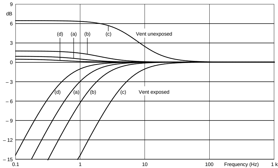
Fig.2.8 The magnitude of the low frequency microphone response is influenced by the ambient pressure. The responses shown are calculated and are all normalized at 250 Hz. They are valid for a microphone which has 10% air-stiffness at nominal ambient pressure (101.3 kPa): a) 1 bar, b) 2 bar, c) 10 bar, d) 0.5 bar
