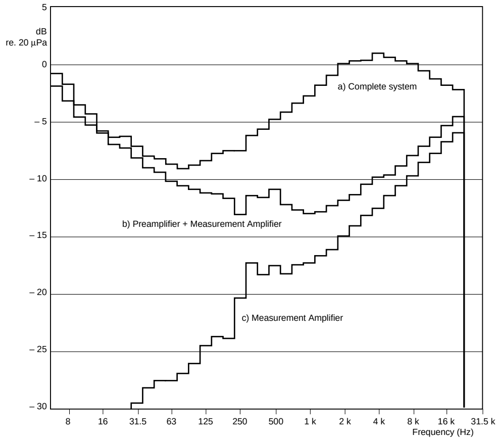
Fig.2.20 Equivalent levels of inherent noise (1/3 octave bandwidth) produced by the elements of a system equipped with a 1" free-field microphone (50 mV/Pa). The microphone, the preamplifier and the measurement amplifier are all significant noise sources in certain parts of the frequency range
