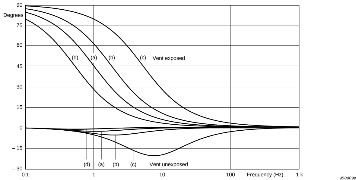
Fig.2.9 The phase of the low frequency microphone response is influenced by the ambient pressure. The calculated responses shown are valid for a microphone which has 10% air-stiffness at nominal ambient pressure (101.3 kPa): a) 1 bar, b) 2 bar, c) 10 bar, d) 0.5 bar
