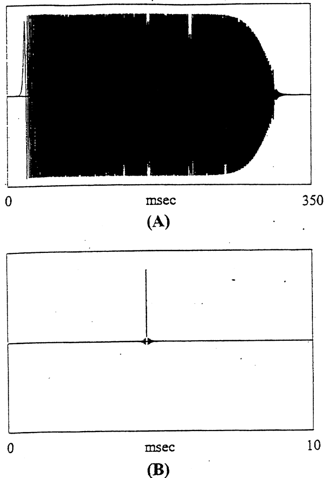
FIG. B1. Waveform of (A) the stretched impulse signal, and (B) the exact impulse wave compressed by the phase shift filter.
