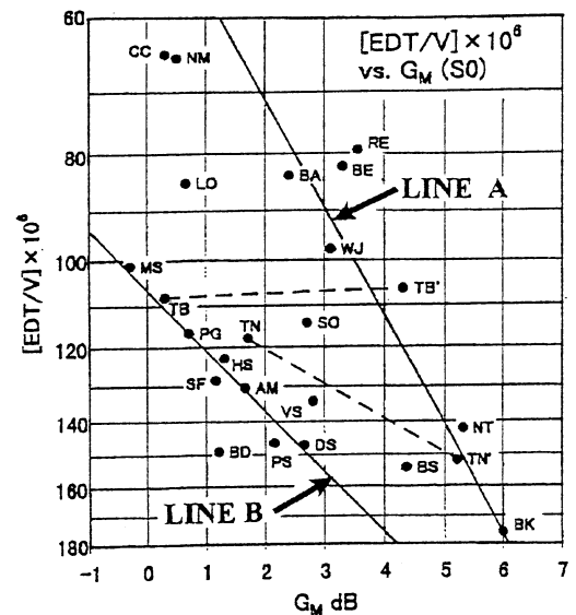
FIG. 8. The early decay time EDT_M divided by the volume V is plotted against the strength factor G_M , both quantities for unoccupied houses with the source at S_0 . The measurements were the average of the positions throughout the audience areas. The houses divide into two groups, with four houses falling between. Line A is taken from Beranek (1996, p. 445) and is for opera houses that, during the measurements, had an orchestra enclosure in place, or a stage set that represented a closed room (with ceiling), or a stage house (fly-tower) that was highly reverberant. Line B is for houses with highly absorbent stage houses and either no stage set or a stage set that allowed free acoustical communication between the stage house and the audience auditorium. The letters TB' and TN' are for measurements made in houses TB and TN with silicated-calcium-board fire curtains down.
