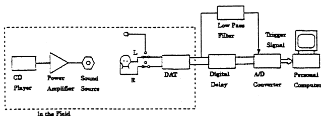
FIG. 1. Block diagram of the measuring system used by the Takenaka R. & D. Institute.
