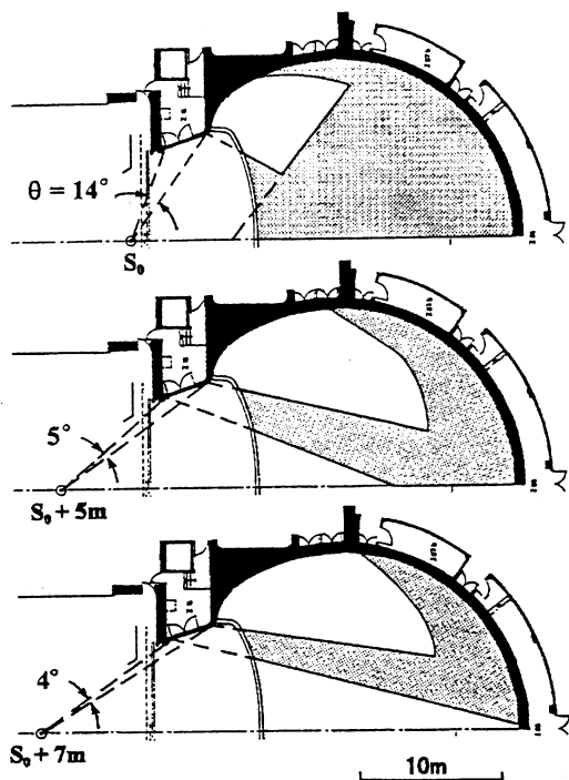
FIG. C1. Area covered by lateral reflections from lower side walls on main floor in Berlin Komischeoper for three source positions: S_0 (upper) and S_0 plus five and seven meters backward (middle and lower). At S_0 , a larger portion of a singer's voice energy ( \theta = 14^\circ ) reaches the main floor audience than reaches there when the singer moves up-stage 5 or 7 m ( \theta = 5^\circ or 4^\circ ). Also, the area covered by the reflected sound decreases.
