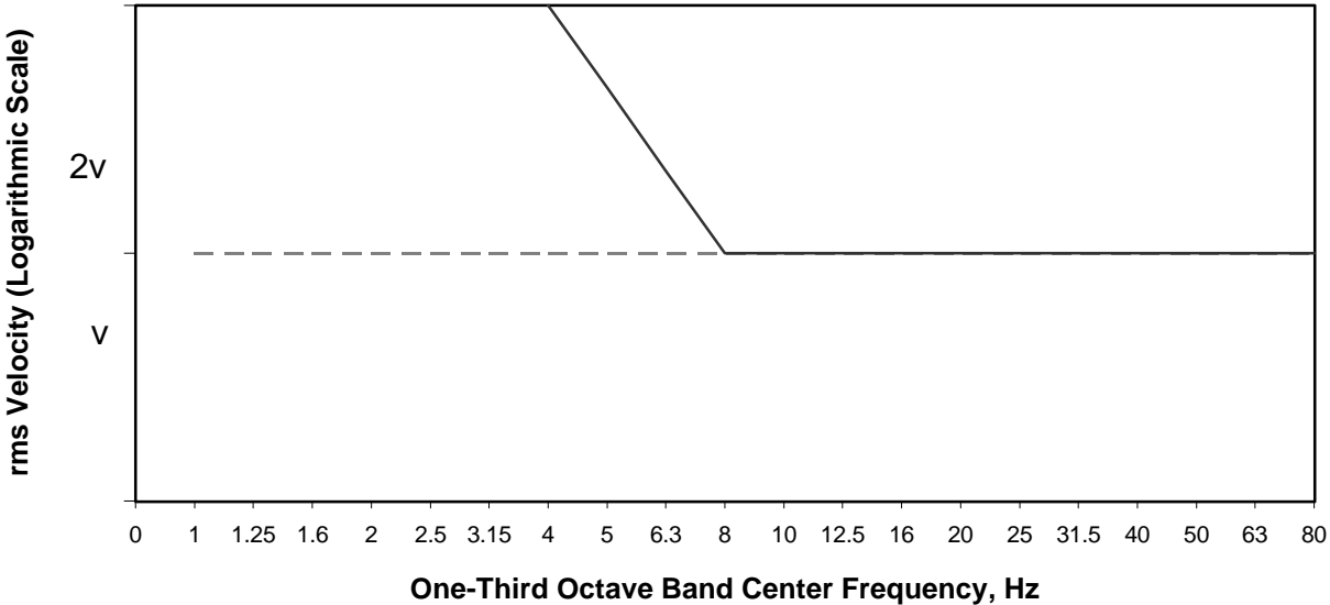
Figure 5: General Criteria Curve Form Suggested by Ungar et. al. (3) to be Used with Values of Table 1. Solid curve pertains to equipment without pneumatically-isolated systems, dashed curve to equipment with low-frequency pneumatic isolation.
