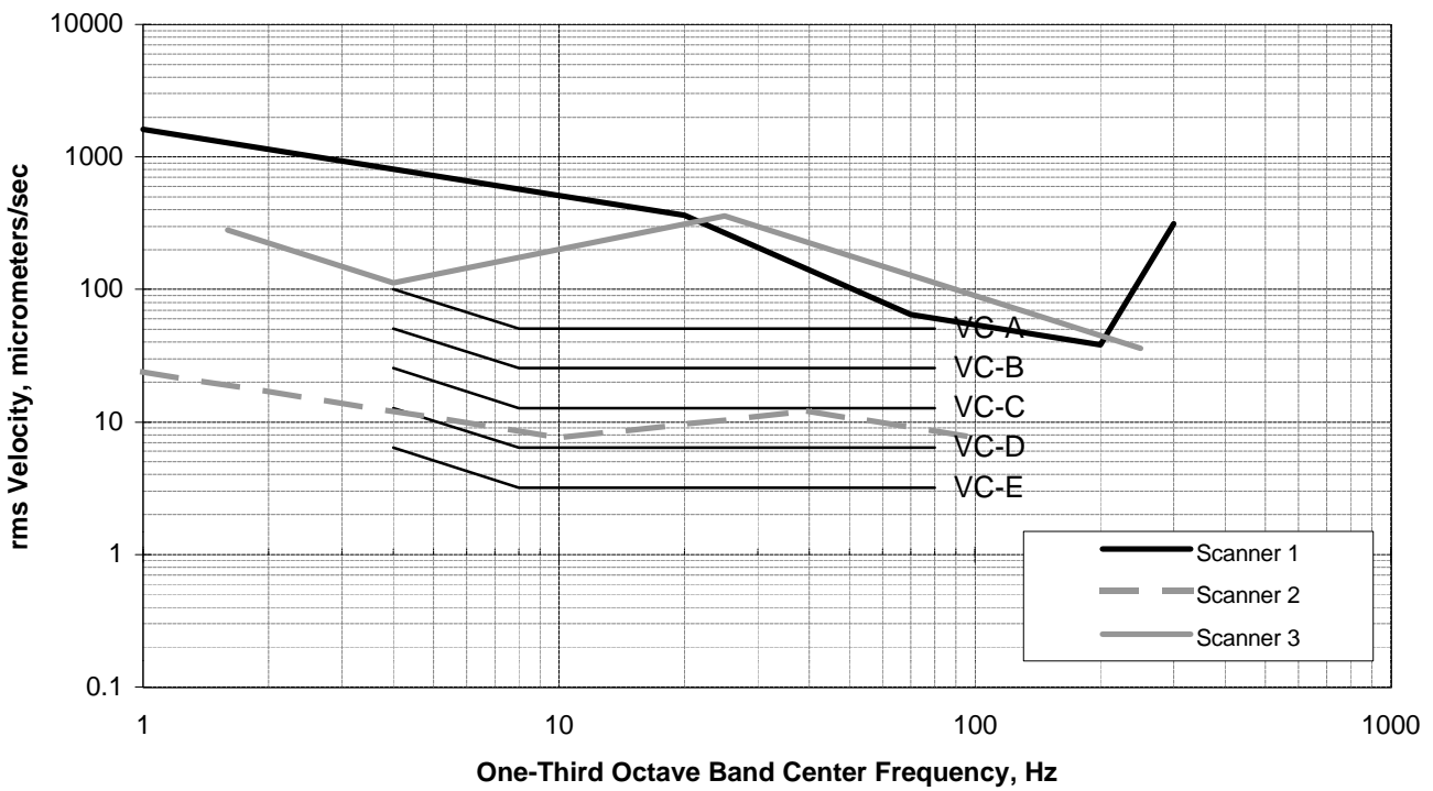
Figure 3: Vibration Specifications for Three Photolithography Scanners versus Generic Vibration Criterion (VC) Curves
