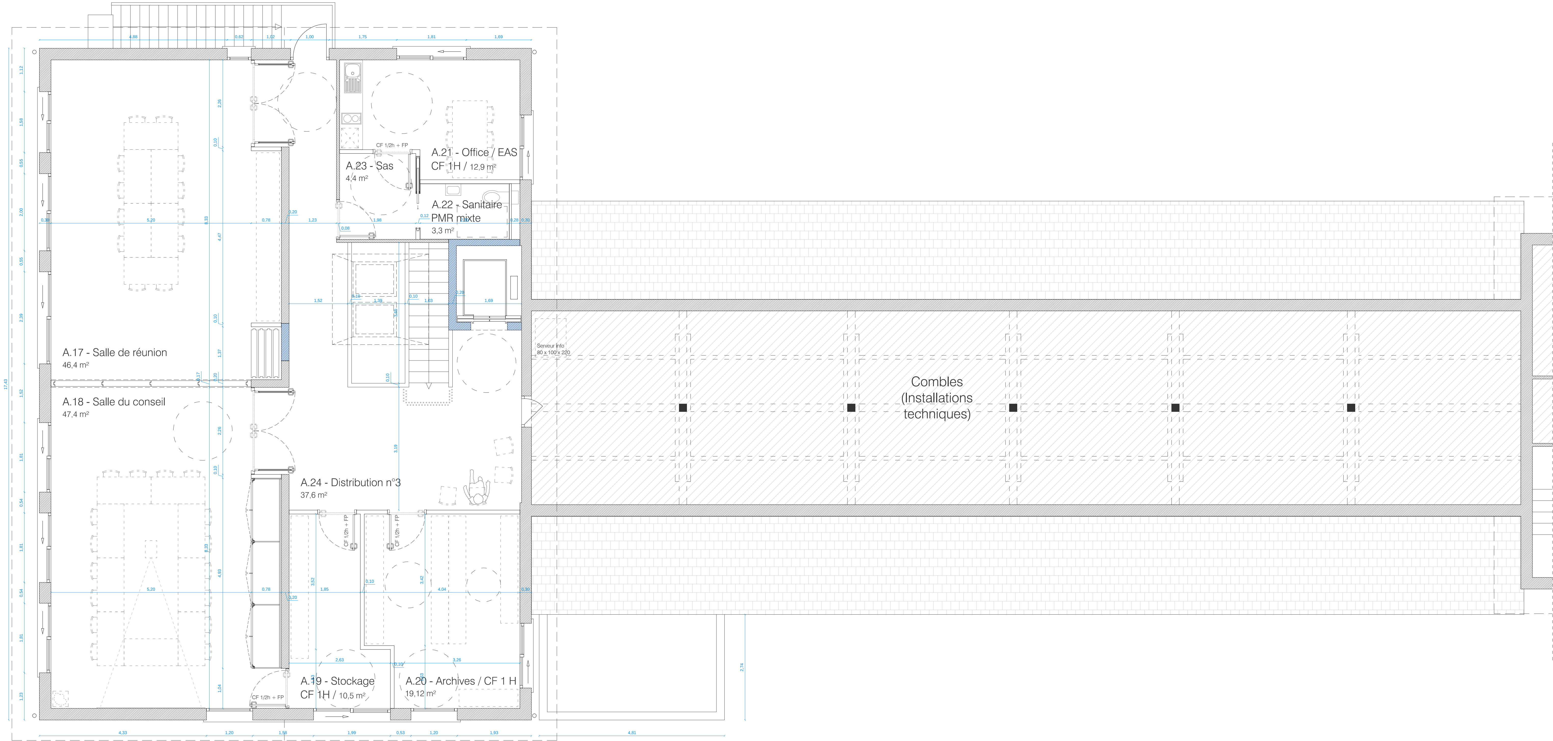
Plan R+1
